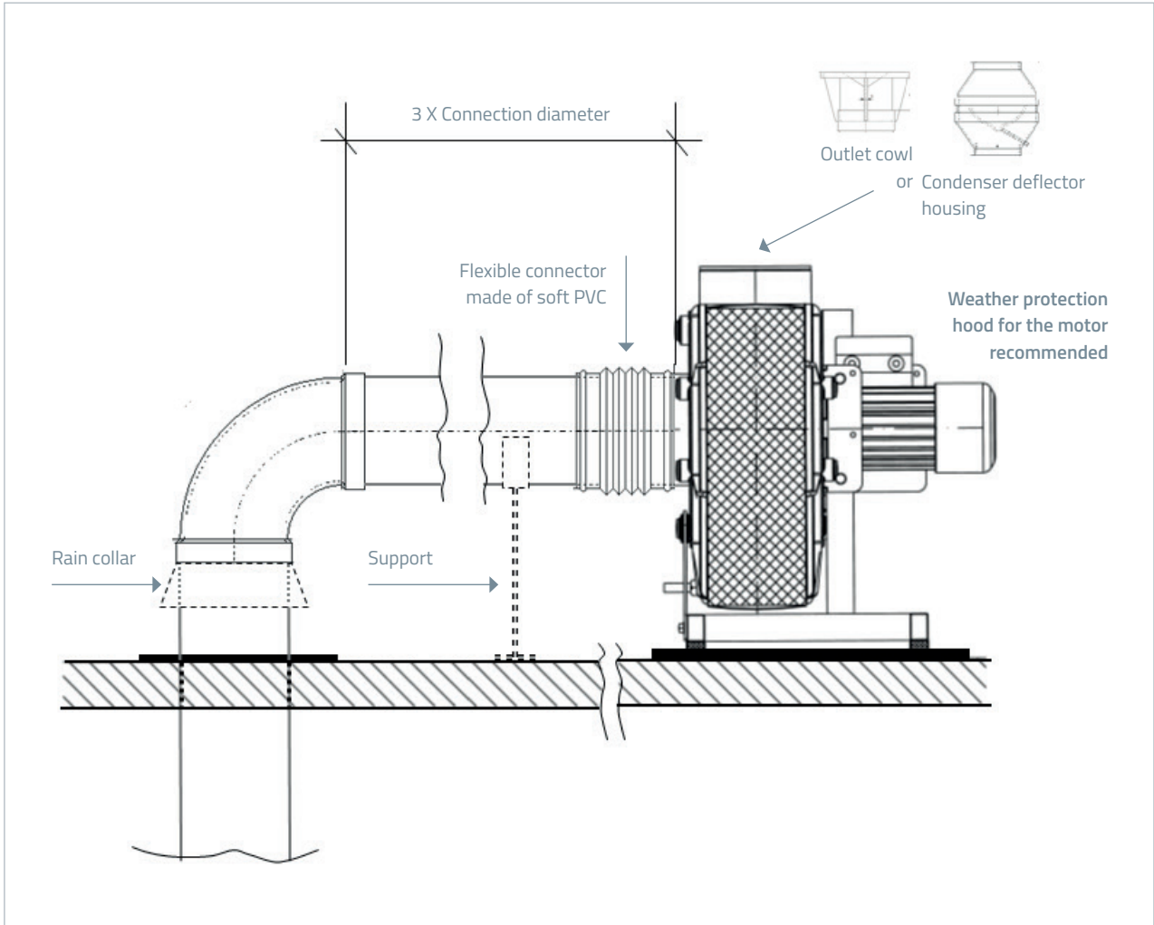
Radial fan as Roof fan
